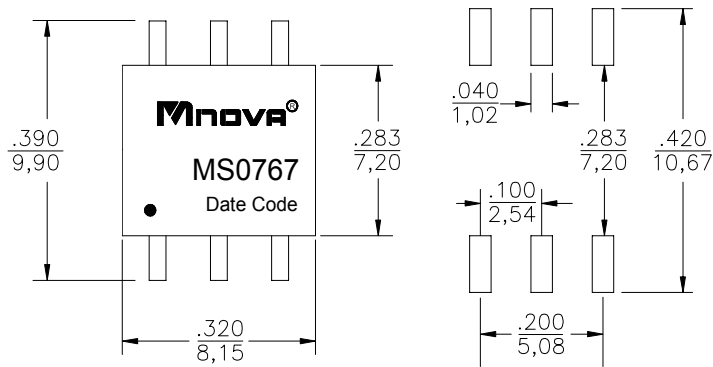
recommend PAD layout
